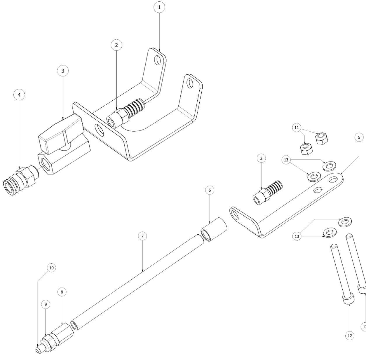
FIG. 1 – Complete Silica Dust Suppression Kit
