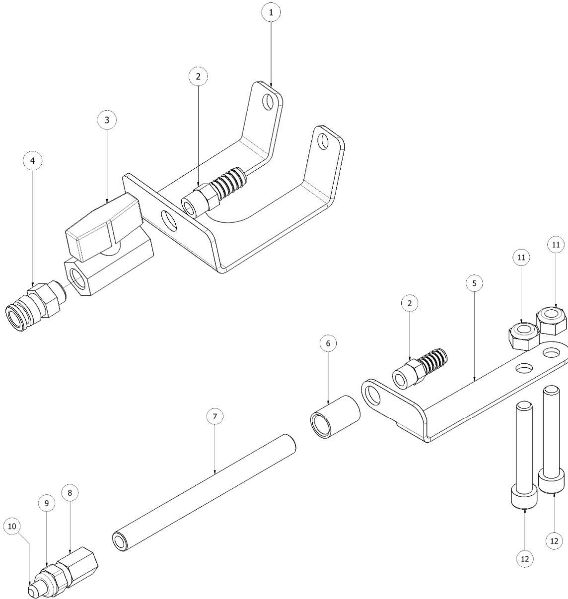
FIG. 1 – Complete Silica Dust Suppression Kit
